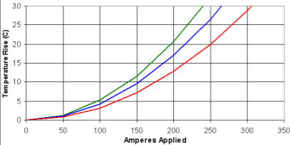
SB350 Fuselok Temperature Rise vs. Applied Current
