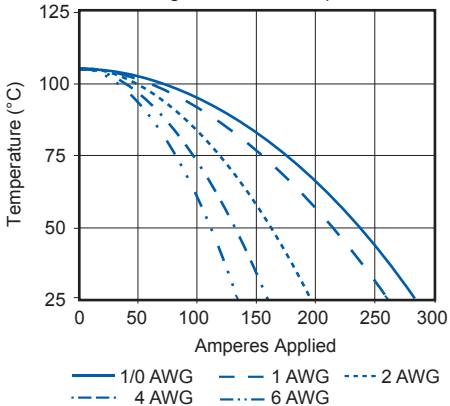
PP120 Singlepole Derating vs. Ambient Temperature
