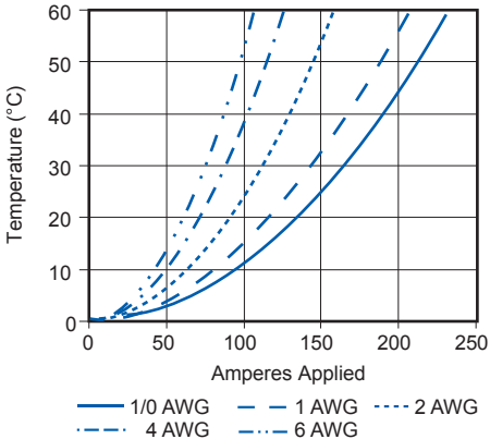
PP120 Multipole Temperature Rise at Constant Current
