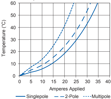
PP25 PCB Temperature Rise at Constant Current
