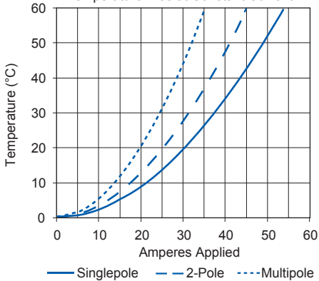
PP45 PCB Temperature Rise at Constant Current
