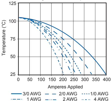
PP180 Singlepole Derating vs. Ambient Temperature
