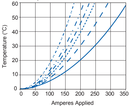
PP180 Singlepole Temperature Rise at Constant Current
