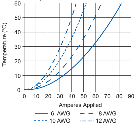
PP75 Multipole Loose Piece Contact Temperature Rise at Constant Current
