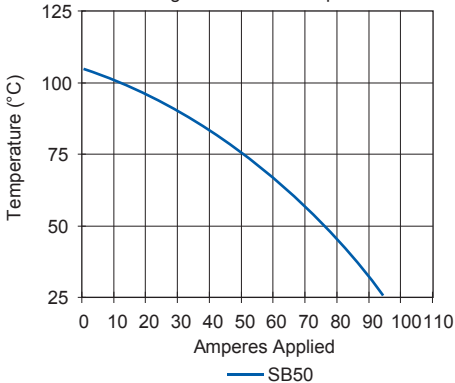
Mini Powerclaw Derating vs. Ambient Temperature
