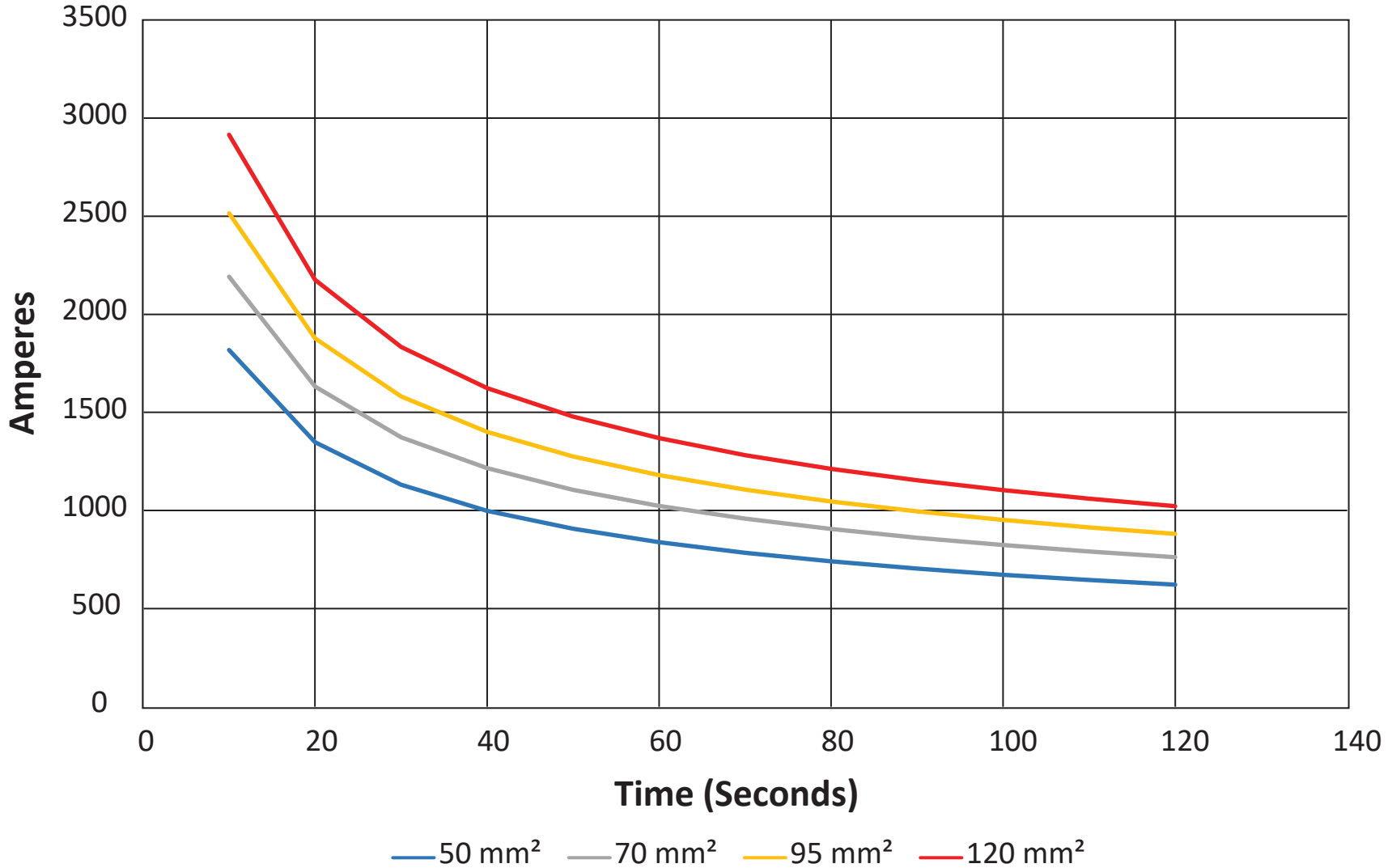
DIN 320 InRush Current Curve - Based on 40°C Rise
